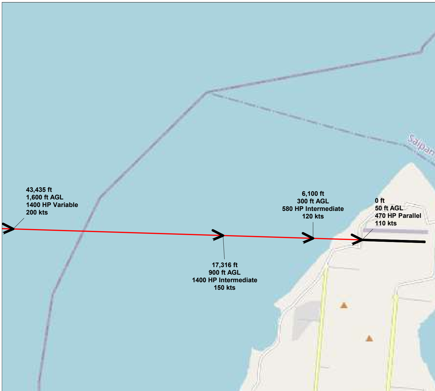
Flight Profile 3131
