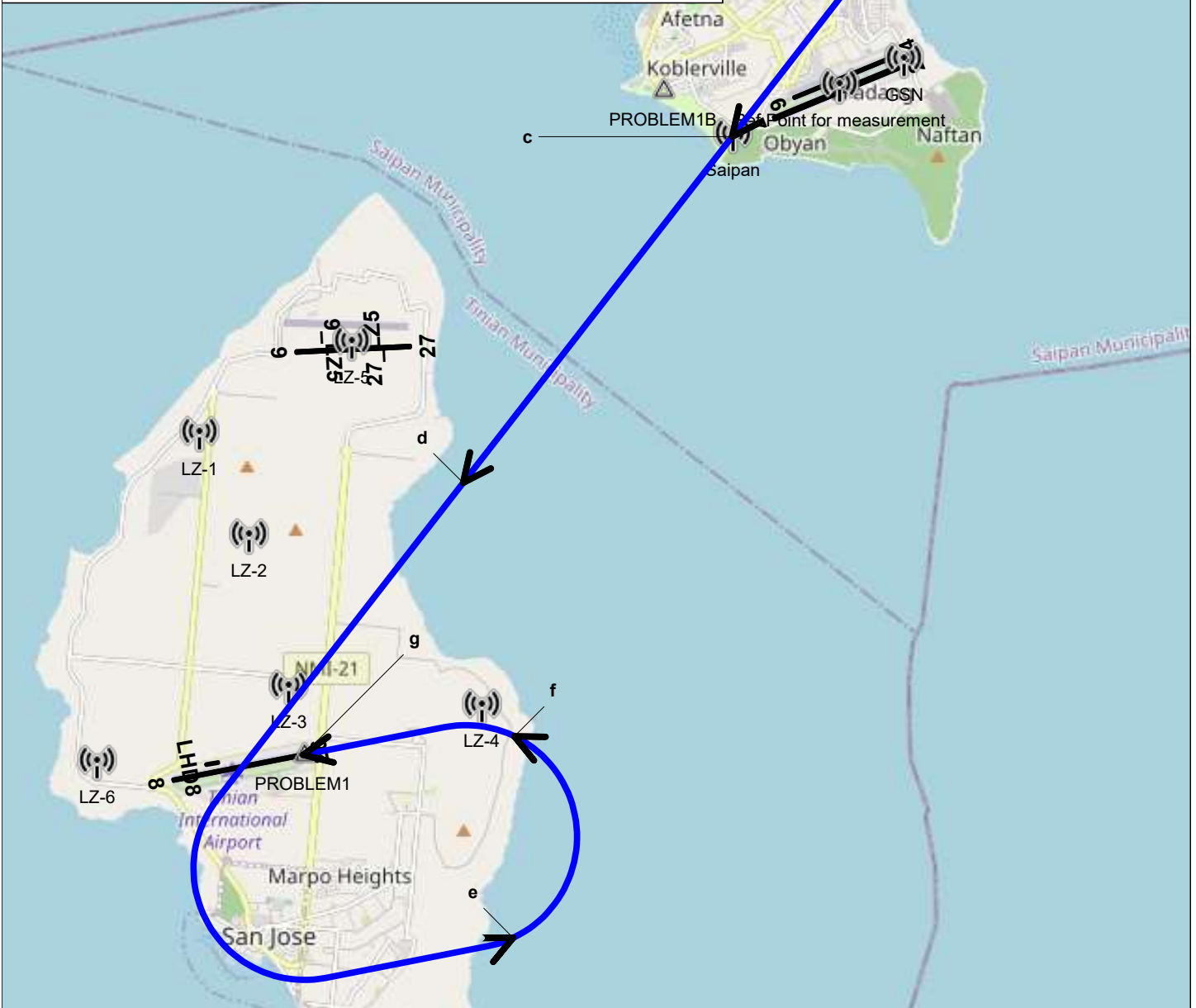
Military Flight Profile KC-135_AF1 Flight Track 26A2_2 - NDB ARRIVAL
